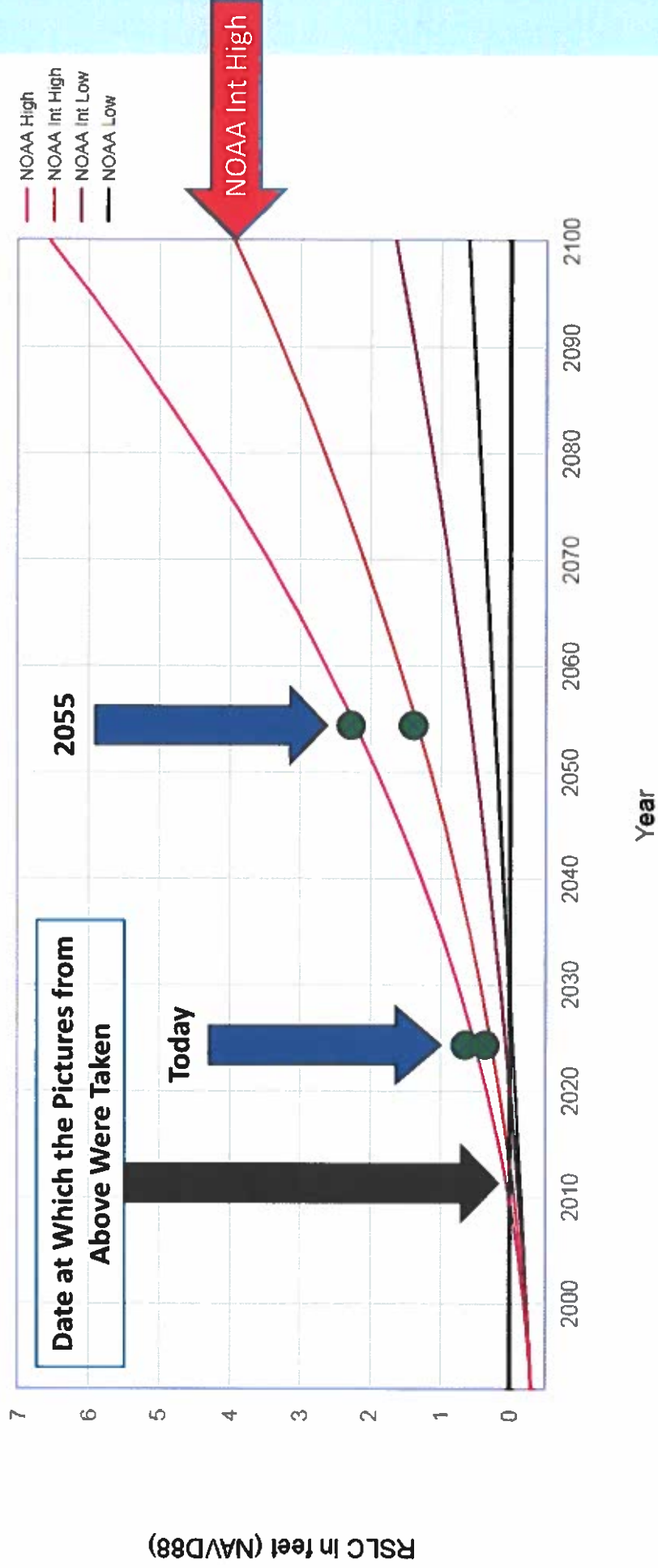
Estimated Relative Sea Level Change Projections - Gauge: 8452560, Newport, RI
